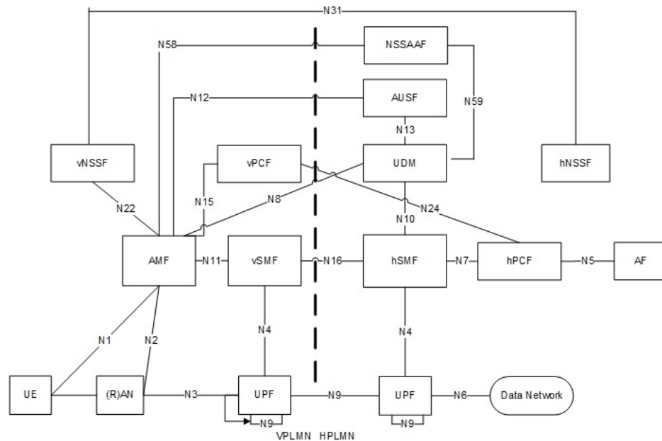
Figure 234: 5G NR HR Roaming Architecture
