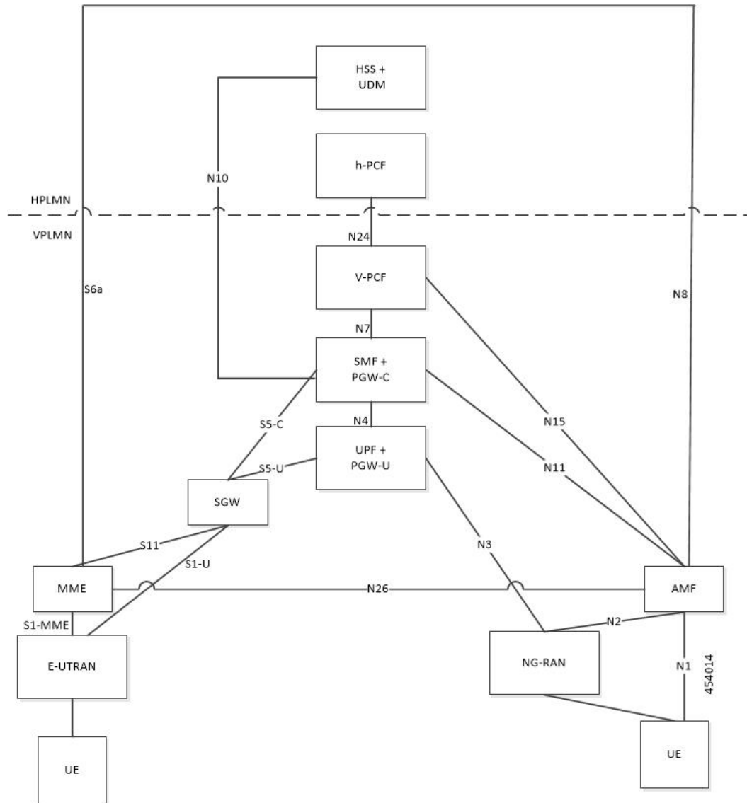
Figure 230: Local Breakout Roaming Architecture for 4G Sessions
