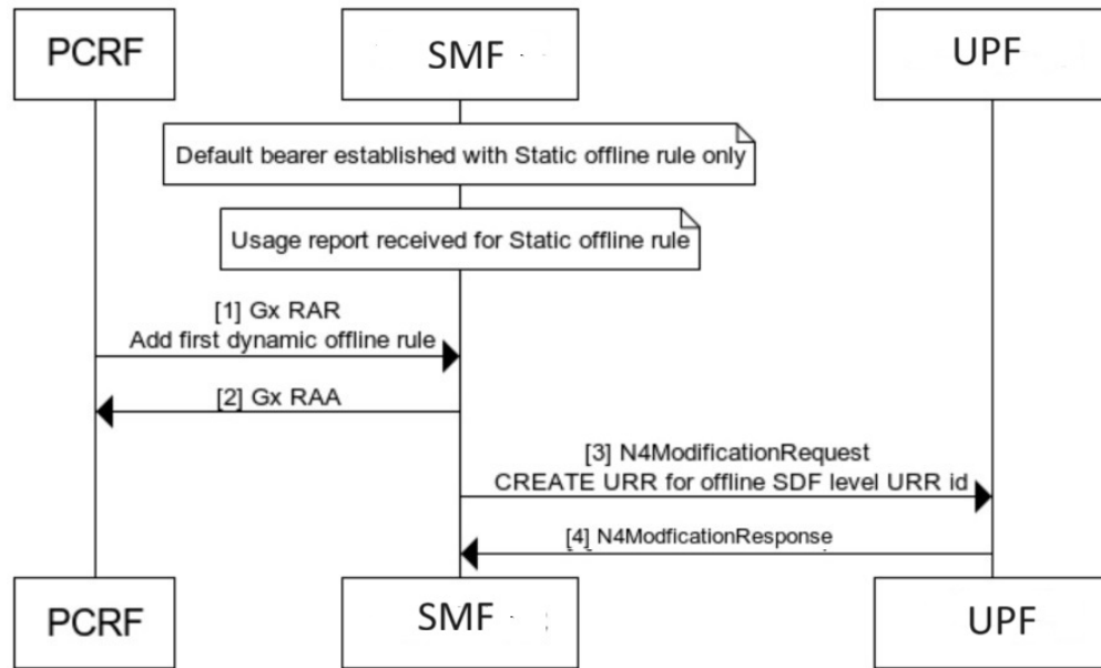
Figure 150: Call Flow for Adding First Dynamic Rule after Usage Report
