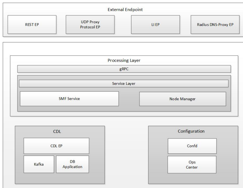
Figure 197: Communication Workflow of Pods
