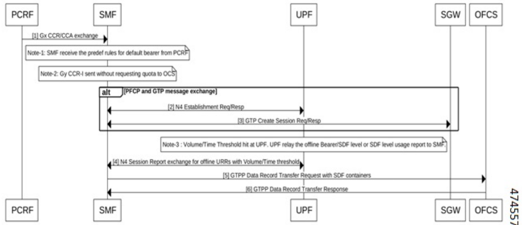
Figure 137: Call Flow for Usage Report in N4 Session Report for Offline Static or Predefined Rules
