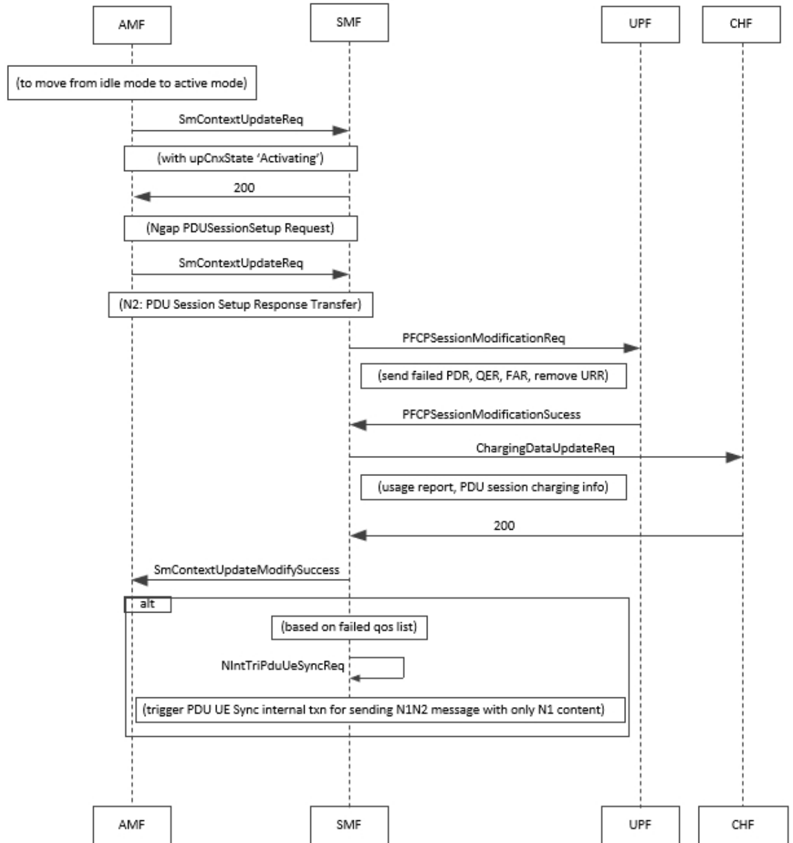
Figure 81: PDUIM Idle to Active Mode
