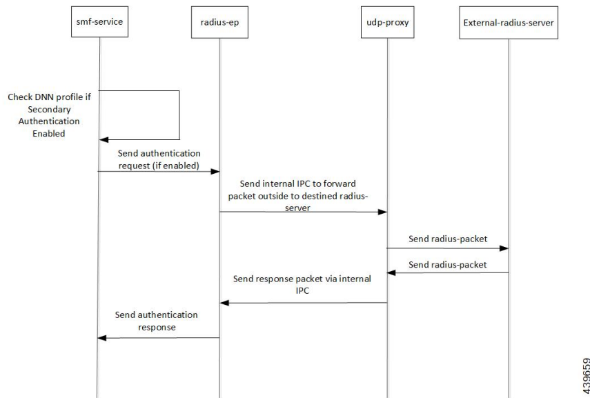
Figure 220: RADIUS Authentication Call Flow
