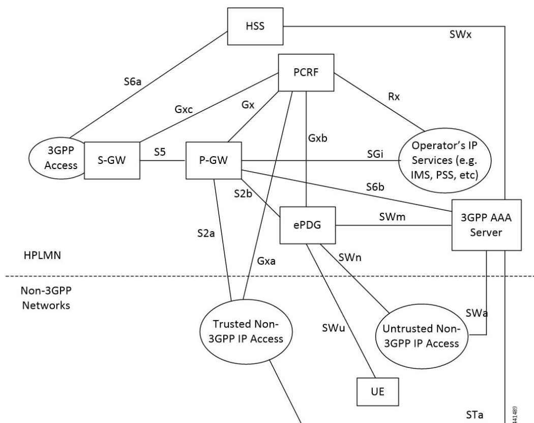
Figure 104: Non-roaming Architecture Within EPS using S5, S2a, and S2b Interfaces
