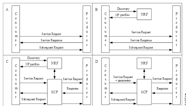
Figure 166: Communication Models for NF and NF Services Interaction
