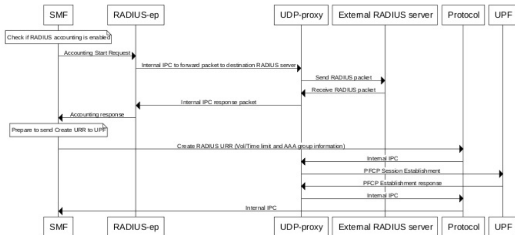
Figure 221: RADIUS Accounting Start Call Flow
