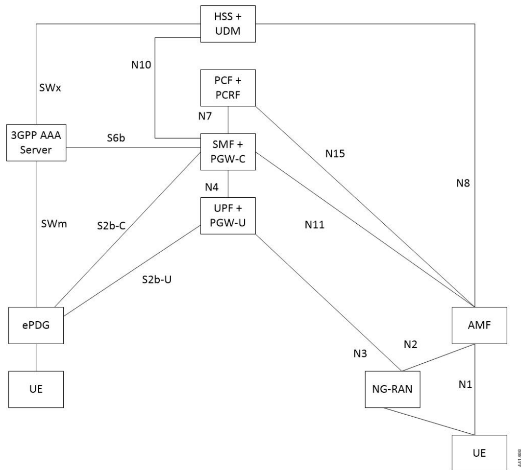
Figure 103: Non-roaming Architecture for Interworking between ePDG or EPC and 5GS
