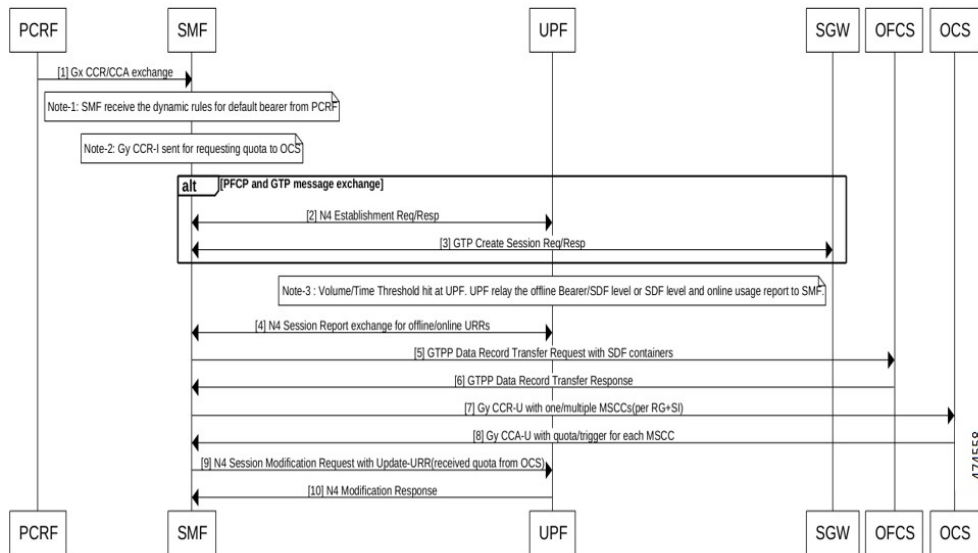
Figure 138: Call Flow for Usage Report in N4 Session Report for Online and Offline
