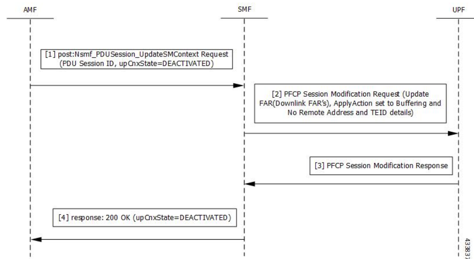
Figure 265: Deactivation of the User Plane Connection Call Flow
