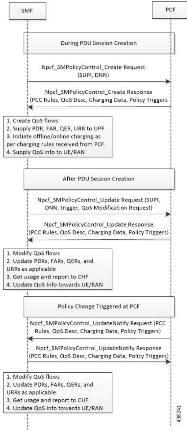
Figure 205: Dynamic Policy Management Call Flow
