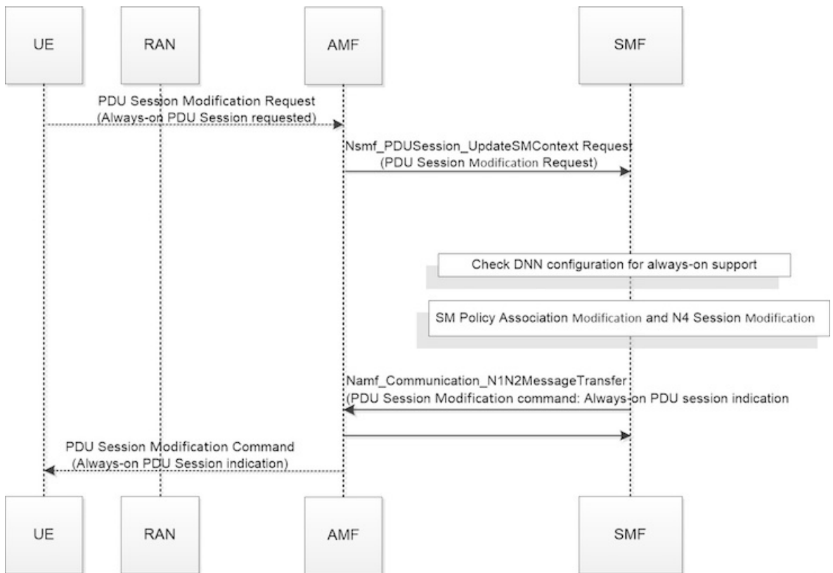
Figure 273: UE-requested PDU Session Modification Call Flow
