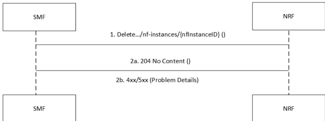
Figure 184: NRF Deregistration Call Flow
