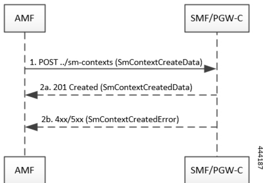
Figure 90: PDU Session in Inactive State
