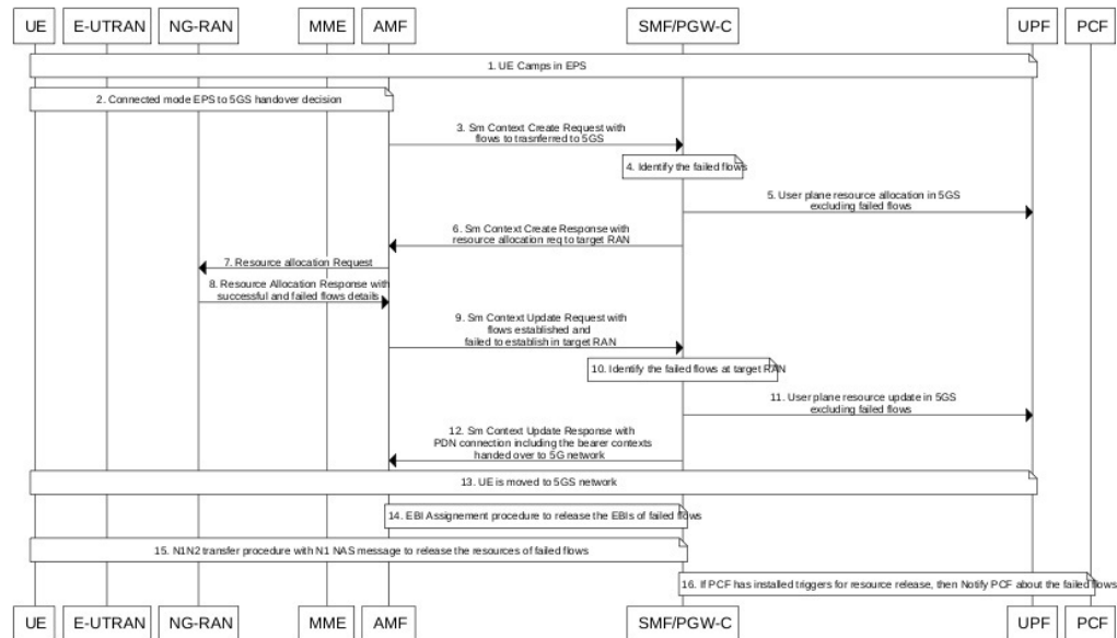
Figure 84: Flow Failure Management Call Flow
