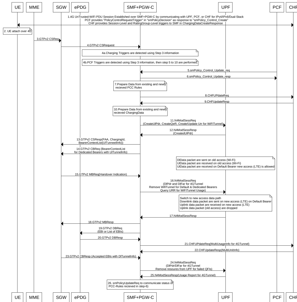
Figure 106: Non-3GPP Untrusted Wi-Fi to EPC Handover Call Flow
