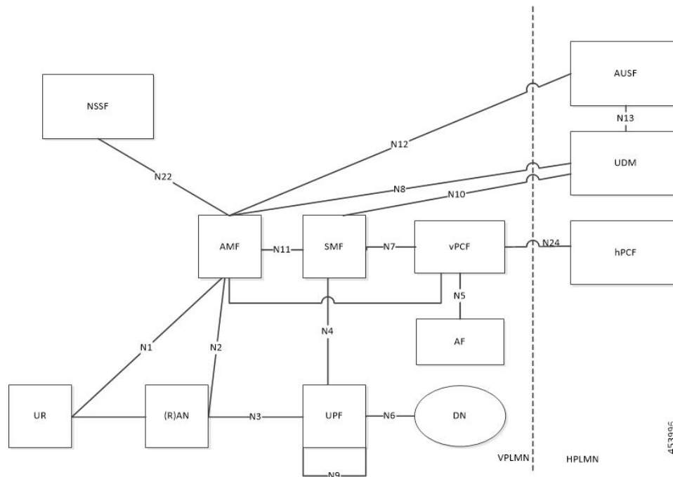
Figure 232: LBO Roaming Architecture for 5G Sessions
