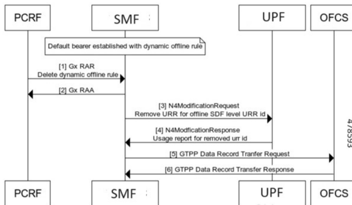
Figure 151: Call Flow for Deleting Rules from Default Bearer
