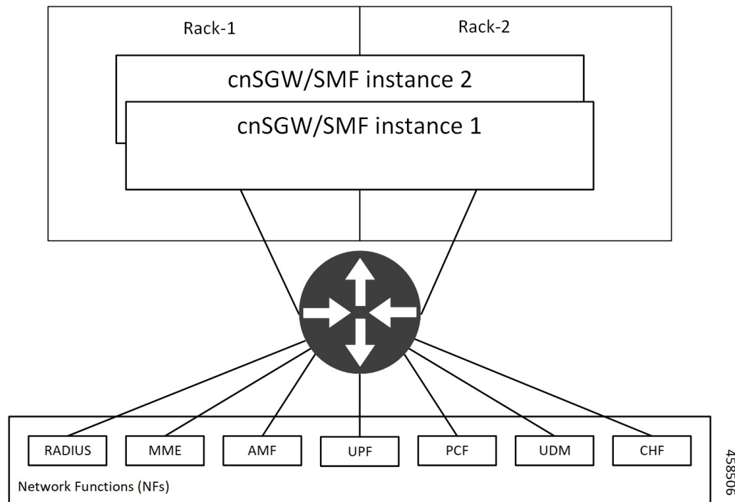
Figure 227: Active-Active Inter-Rack Redundancy Deployment
