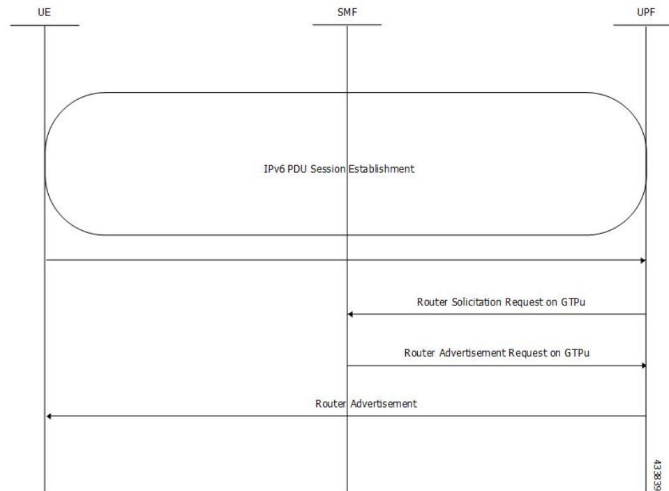
Figure 181: Router Solicitation and Advertisement Message Processing Call Flow
