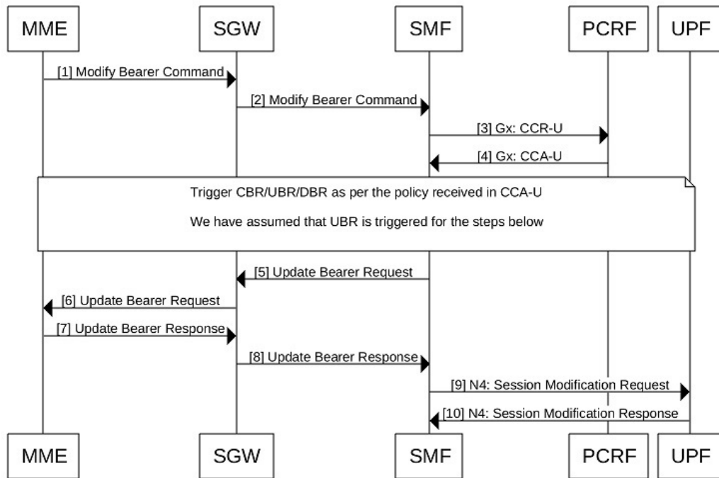
Figure 57: Call Flow for HSS Initiated Bearer QoS Modification
