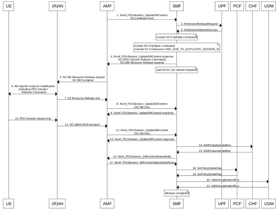
Figure 65: AMF-initiated PDU Session Release with N11 Release=True
