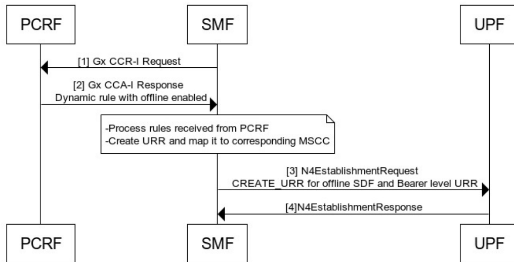
Figure 133: Call Flow for PDN Attach with Only Offline Rules
