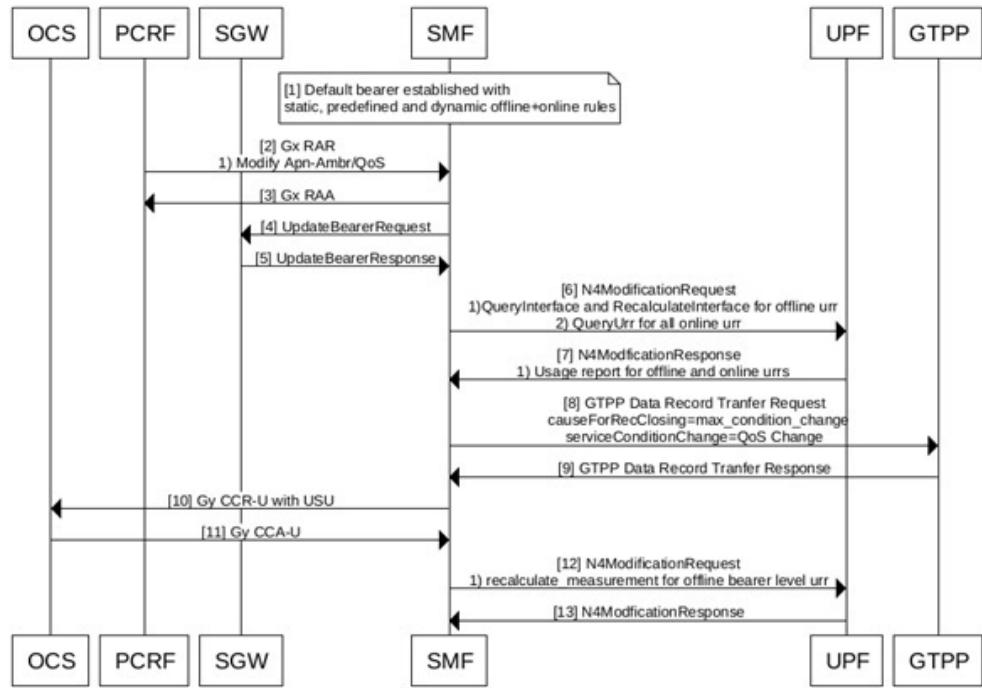
Figure 153: Call Flow for Offline and Online Rules Change
