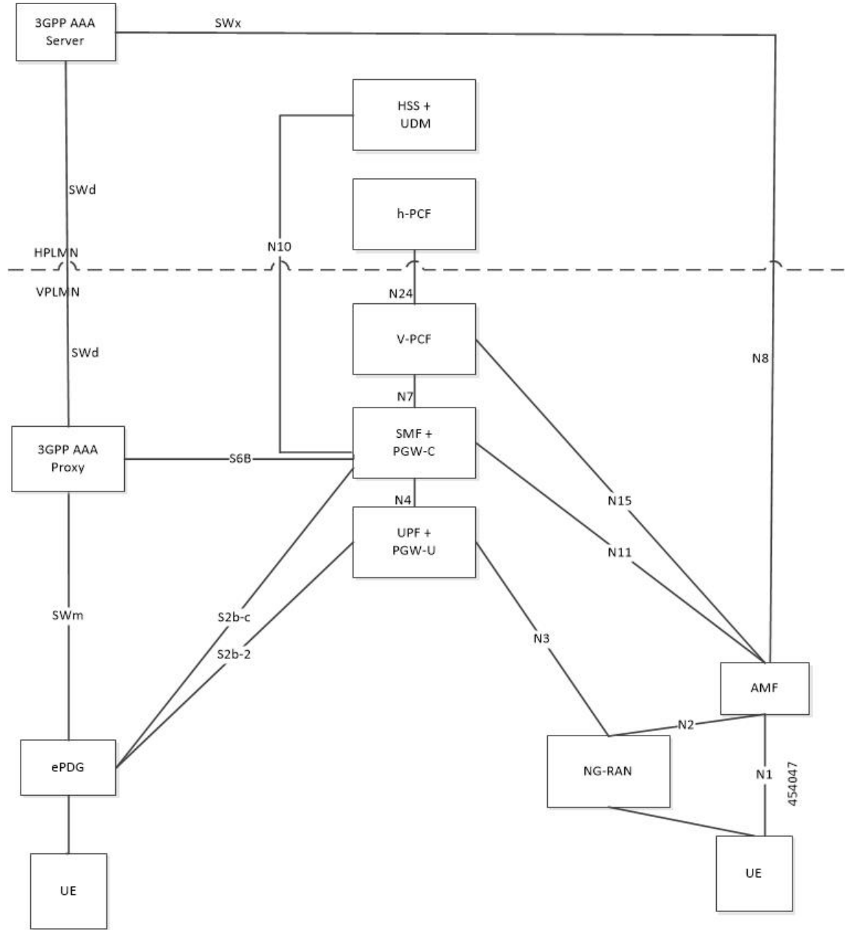
Figure 231: Local Breakout Roaming Architecture for Wi-Fi Sessions
