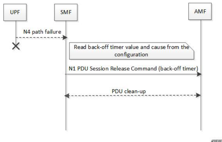
Figure 254: N4 Path Failure Handling Call Flow for Non-roaming Session
