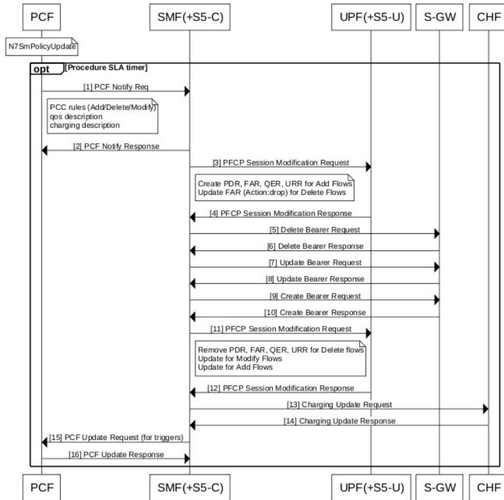
Figure 71: PCF-initiated Modification Call Flow
