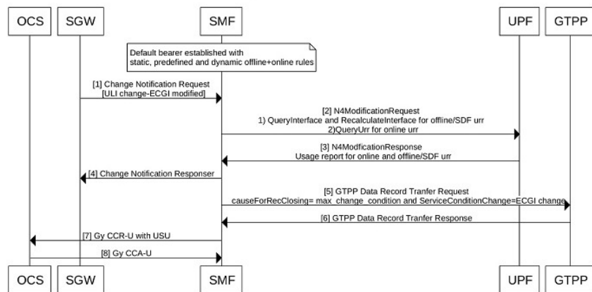
Figure 147: Call Flow for Change Notification
