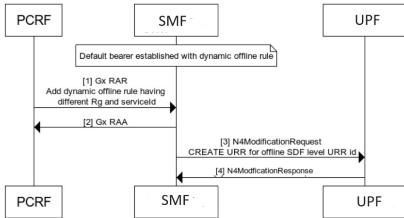
Figure 148: Call Flow Adding Offline Rules to Default Bearer
