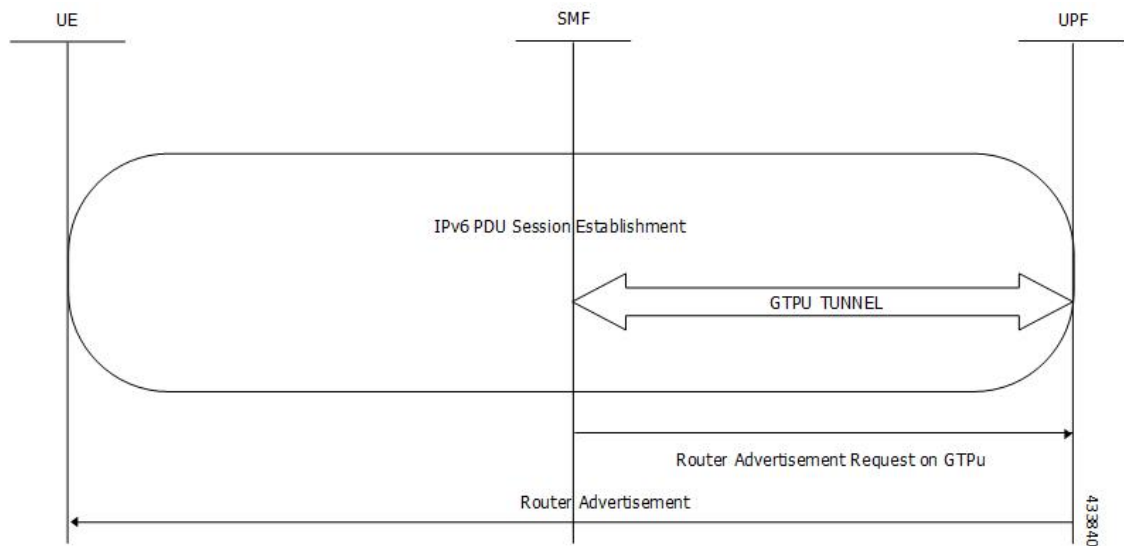
Figure 180: Router Advertisement Message Processing Call Flow
