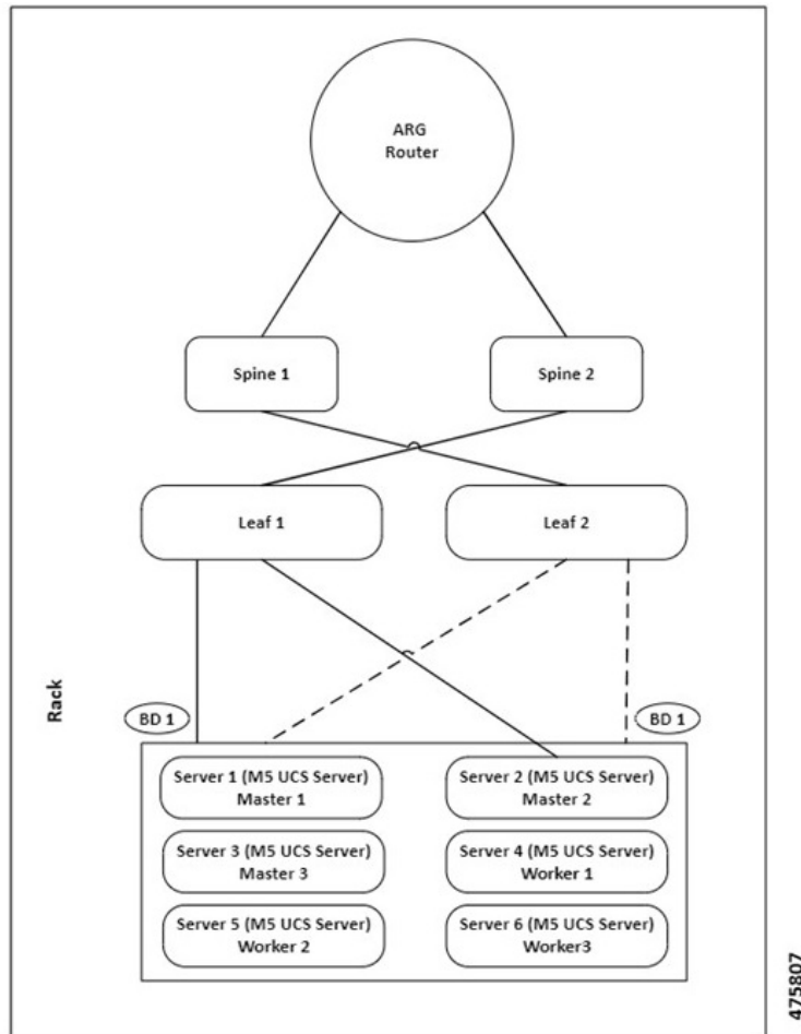
Figure 225: High Availability Layout
