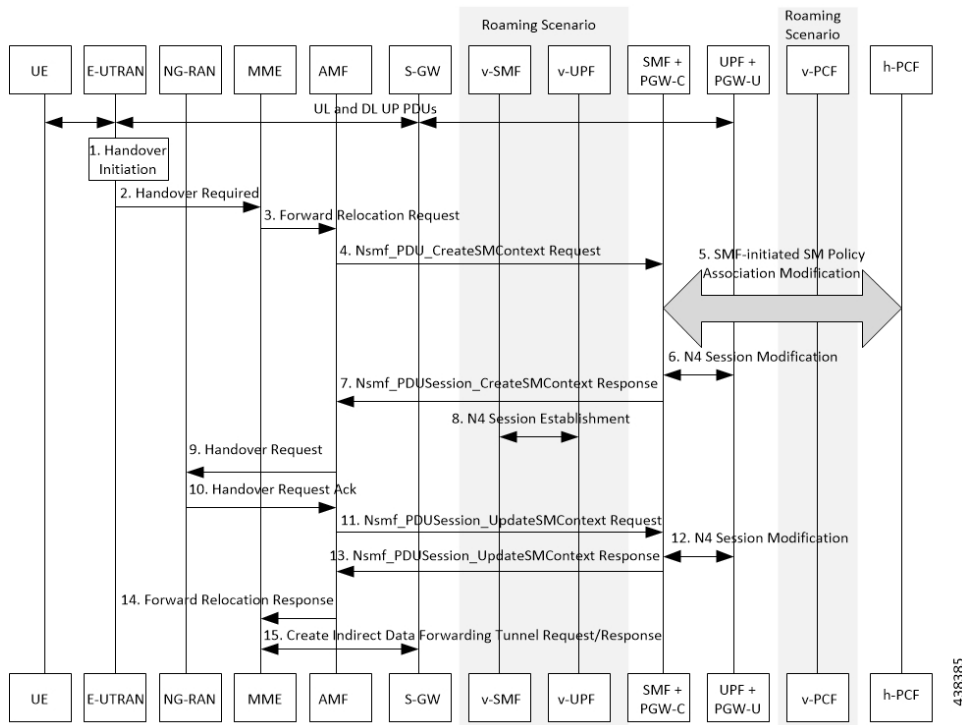
Figure 242: Call Flow for the EPS to 5G Handover Using the N26 Interface
