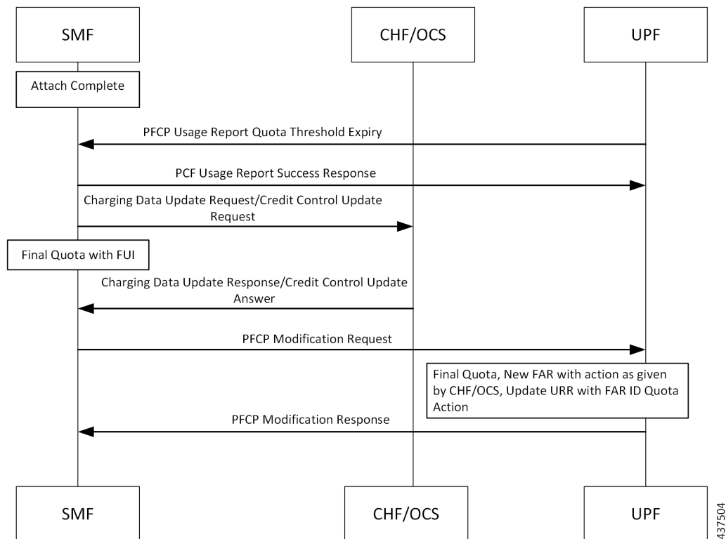
Figure 261: FUI in the Charging Data Initial or Update Response from CHF
