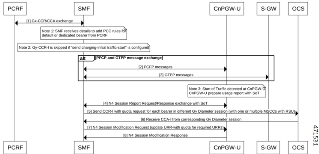
Figure 126: Usage Report with SoT – CCR-I Message Not Sent During Initial Attach or Bearer Creation
