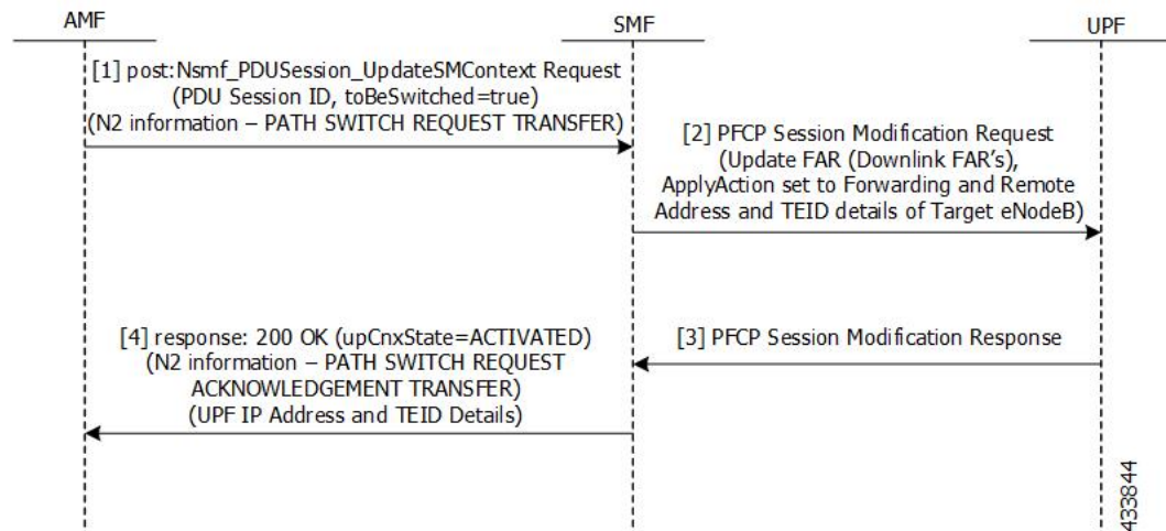
Figure 100: Xn Handover Without UPF Relocation Call Flow
