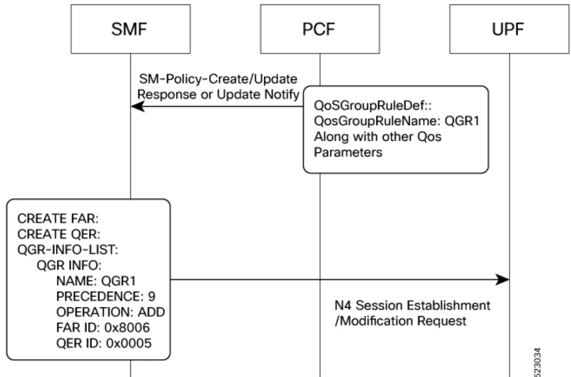
Figure 216: Qos-Group-of-Ruledef Activation Call Flow
