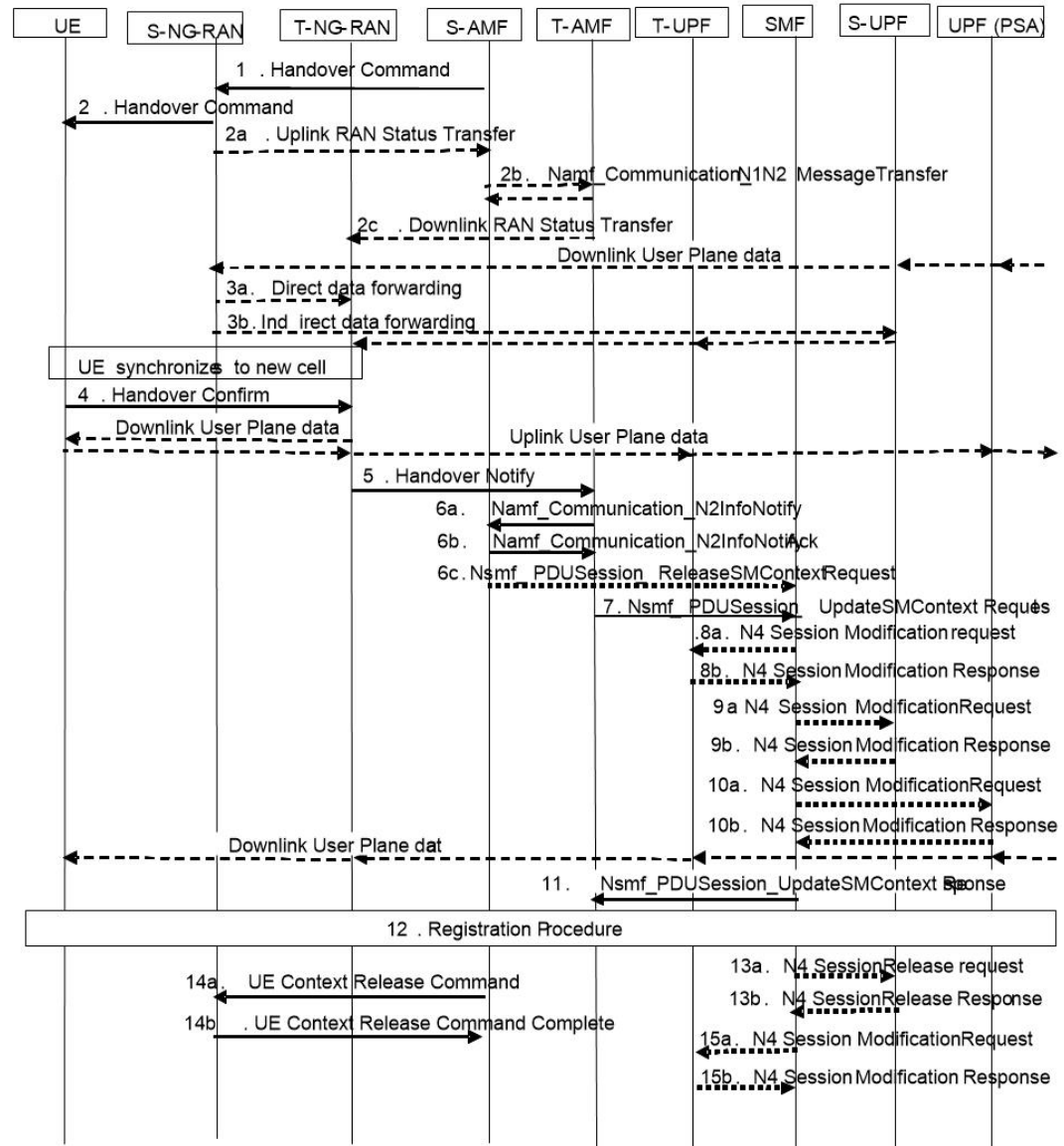
Figure 102: Inter NG-RAN Node N2-based Handover - Execution Phase
