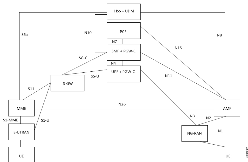
Figure 87: Network Architecture for the EPS-5G Core Interworking
