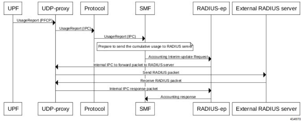
Figure 223: Asynchronous Accounting Interim-Update Call Flow
