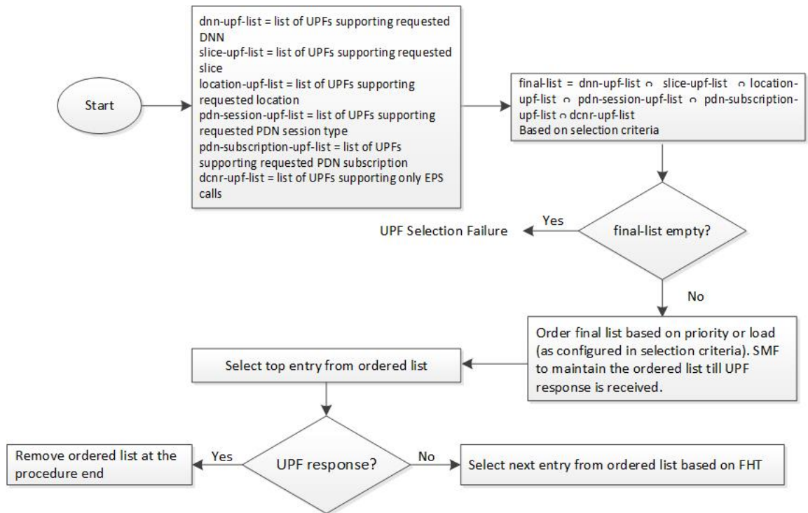
Figure 208: UPF Node Selection Workflow
