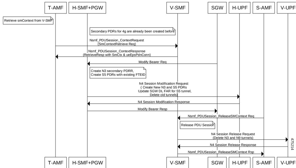
Figure 250: Call Flow for Inter-plmn HO from 5G Roamer to 4G Homer
