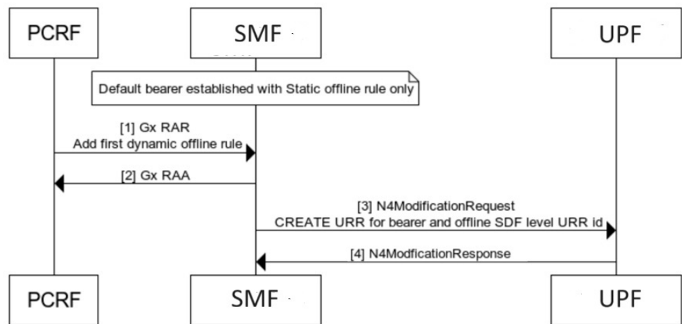
Figure 149: Call Flow for First Dynamic Rule
