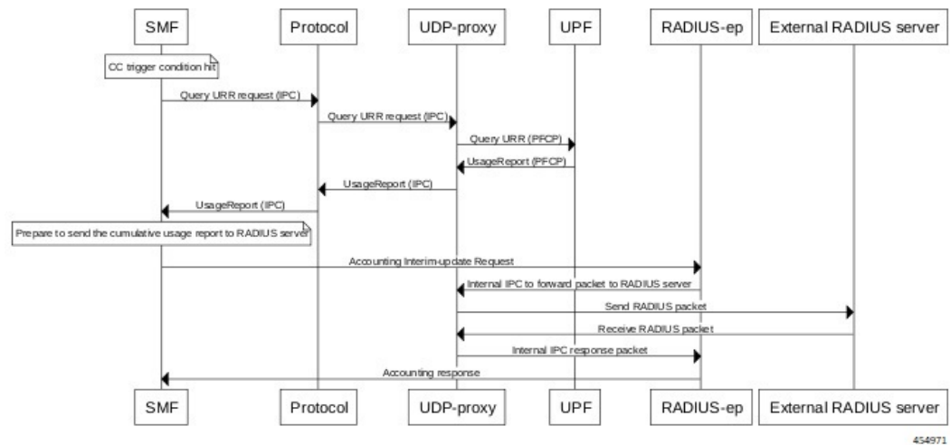
Figure 224: Synchronous Accounting Interim-Update Call Flow
