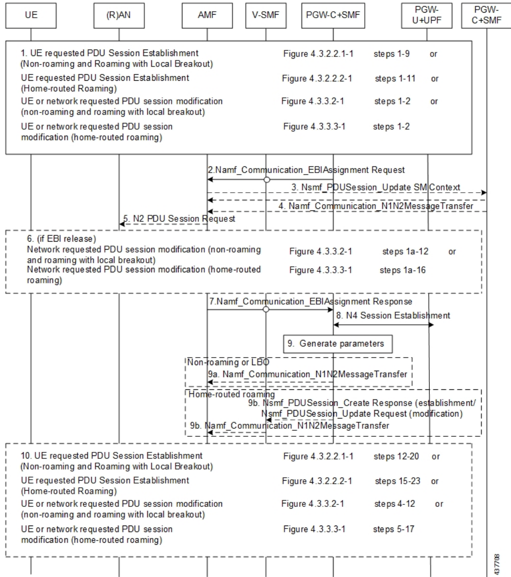
Figure 67: EPS Bearer ID Allocation Call Flow
