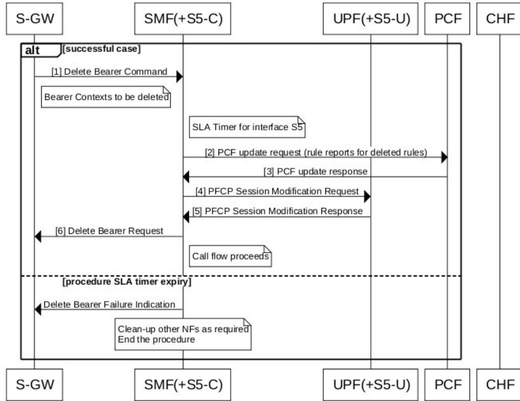
Figure 72: MME-initiated Deletion Call Flow
