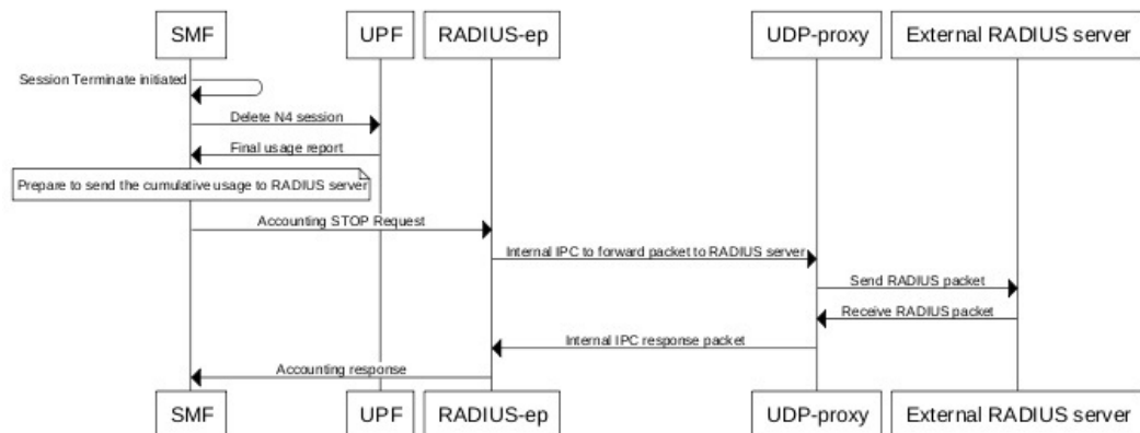
Figure 222: RADIUS Accounting Stop Call Flow
