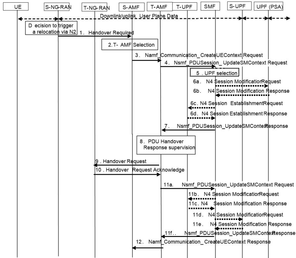
Figure 101: Inter NG-RAN Node N2-based Handover - Preparation Phase
