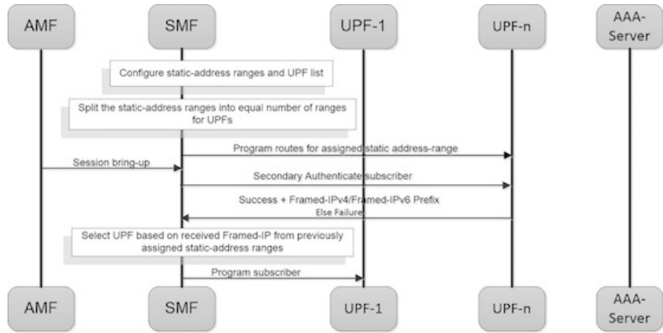
Figure 169: Static IP Call Flow
