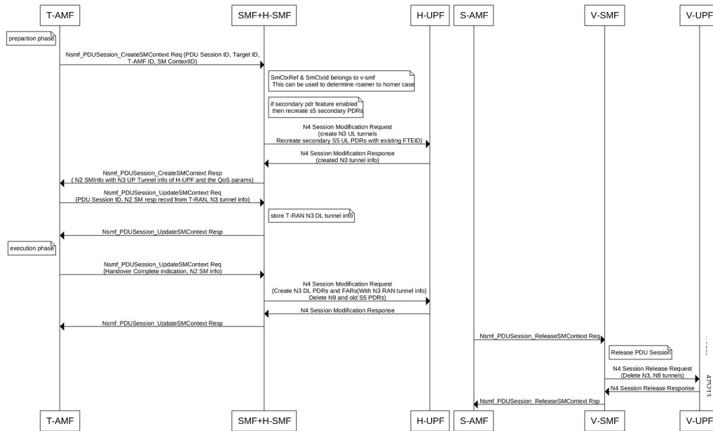
Figure 248: Call Flow for Inter-plmn N2 HO with v-SMF Deletion
