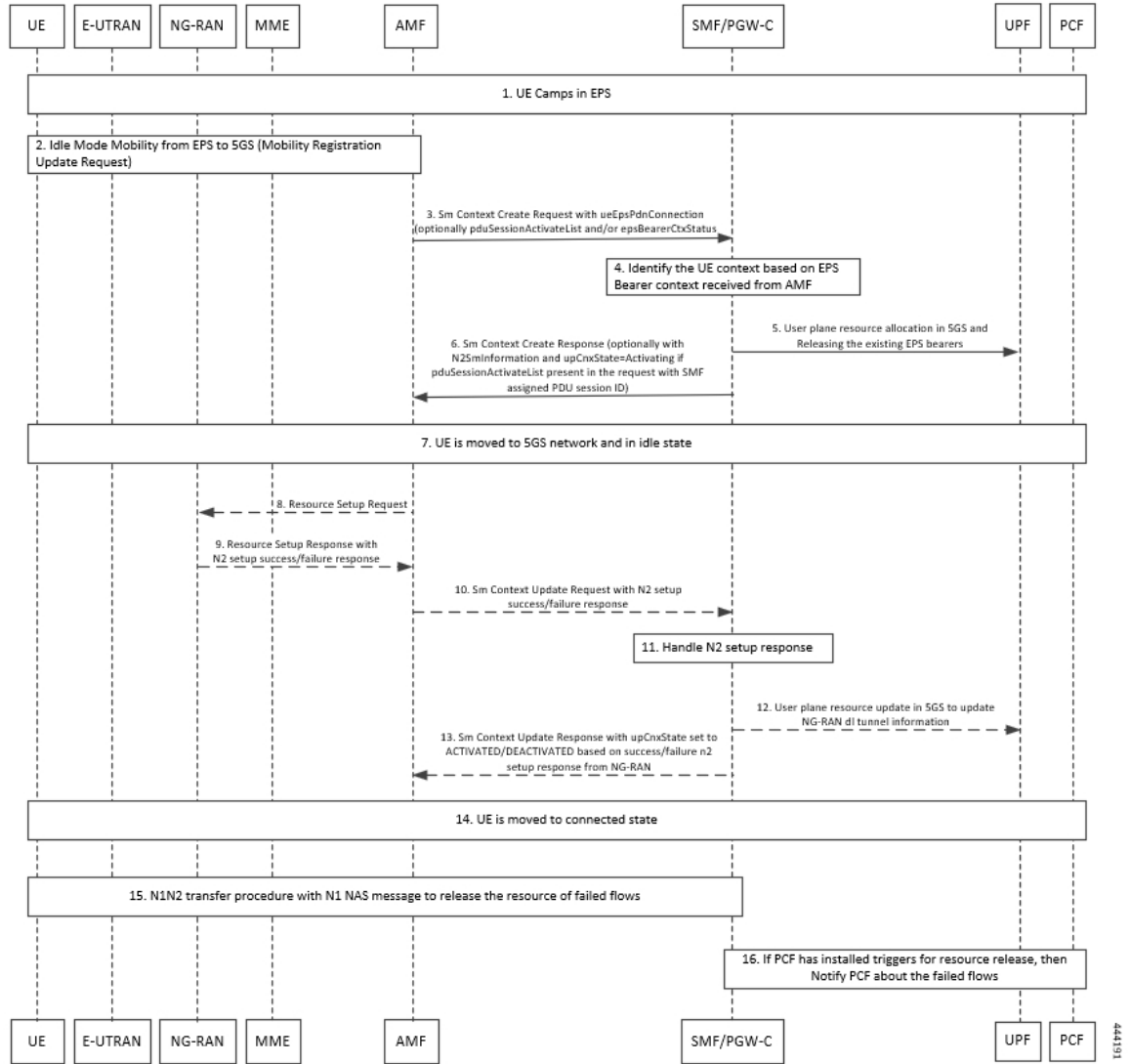
Figure 92: Message Flow across 5GS NEs and Subscriber
