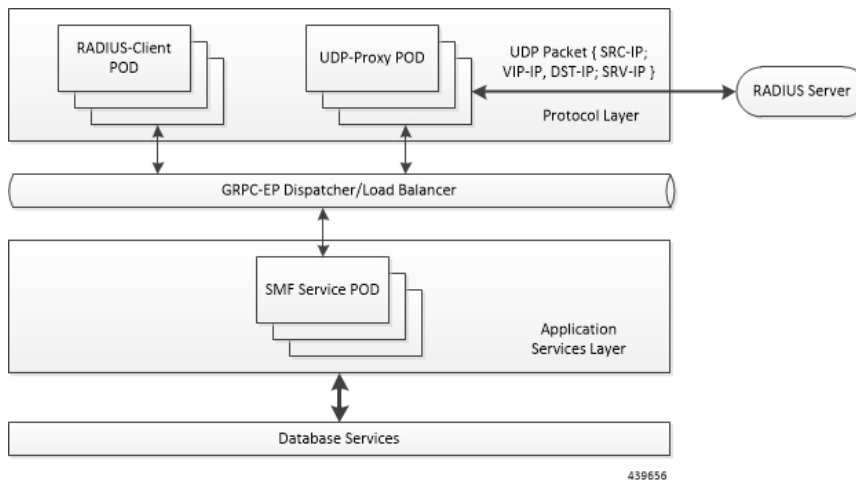
Figure 219: RADIUS Client Integration
