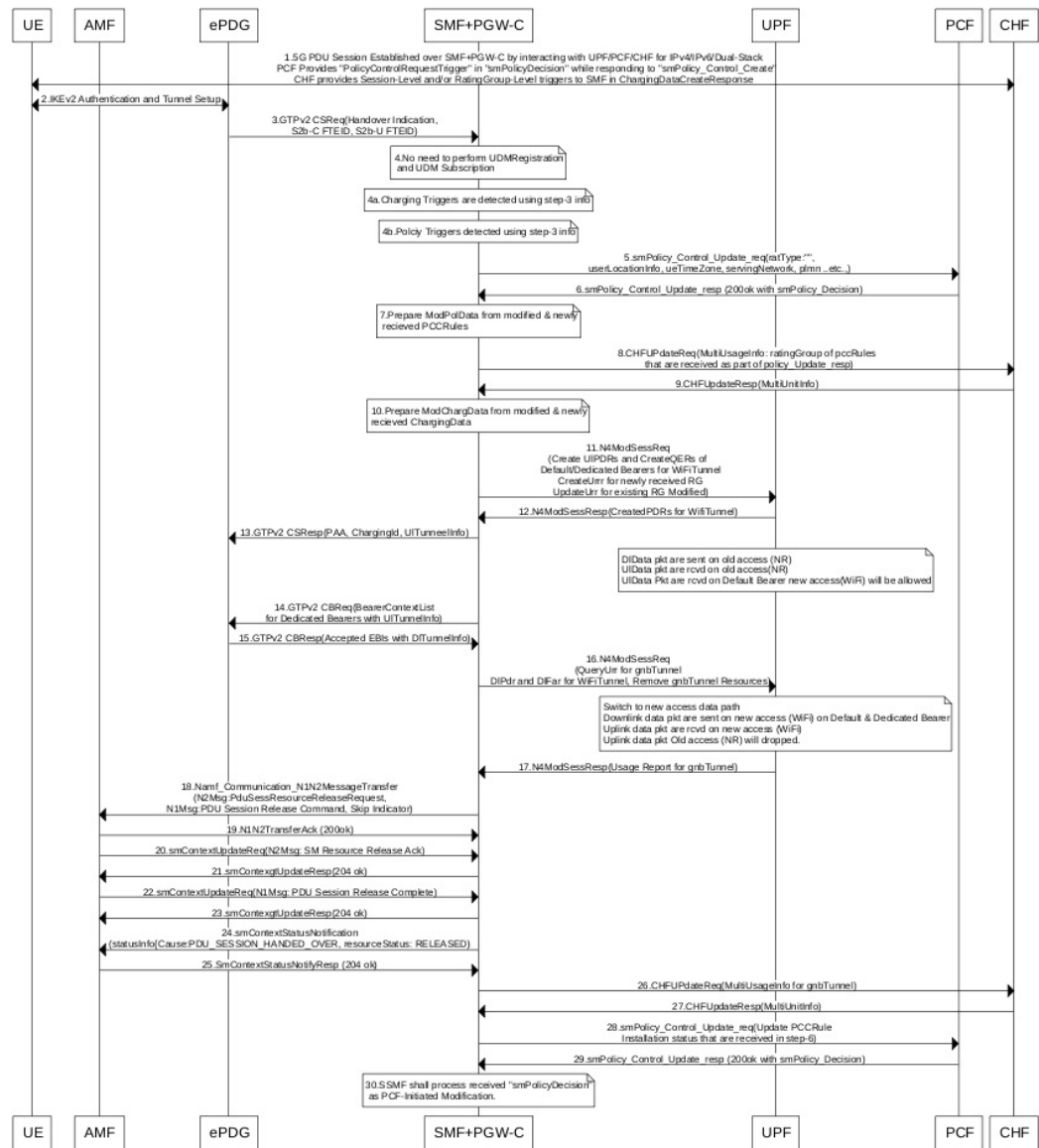
Figure 109: 5GS to Non-3GPP Untrusted Wi-Fi Handover Call Flow
