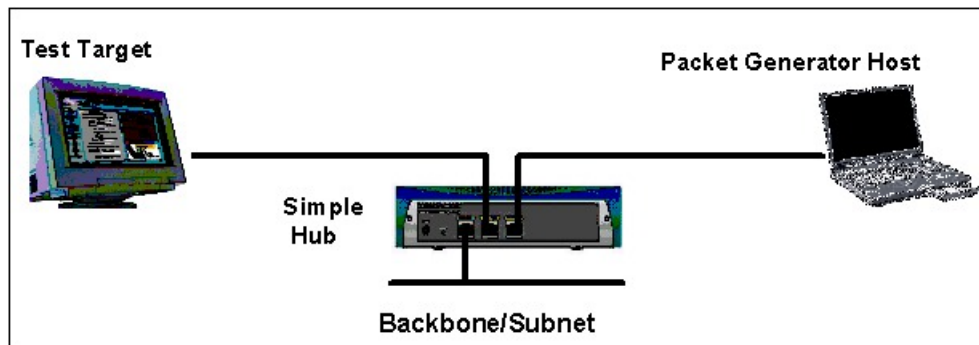
Figure 12: Silent Monitor Ethernet Card Test Configuration
