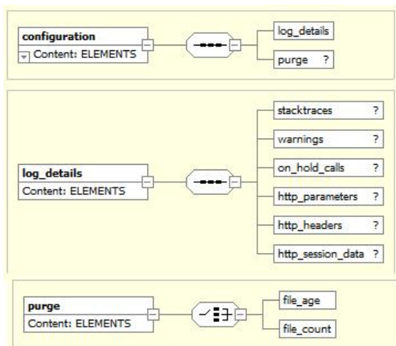
Figure 10: Global Error Log Configuration
