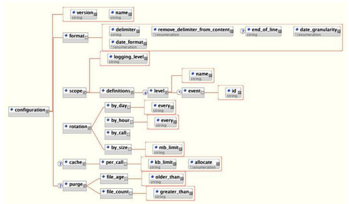
Figure 11: Activity Logger Configuration File Format
