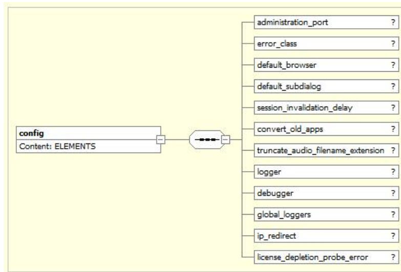
Figure 13: Global Configuration Options
