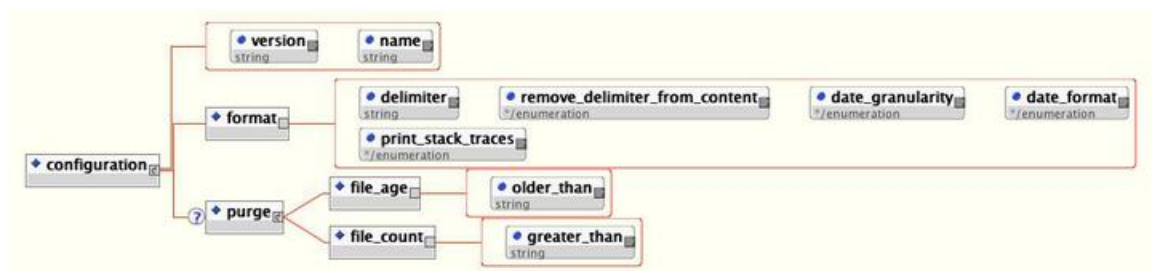
Figure 12: Error Logger Configuration Format
