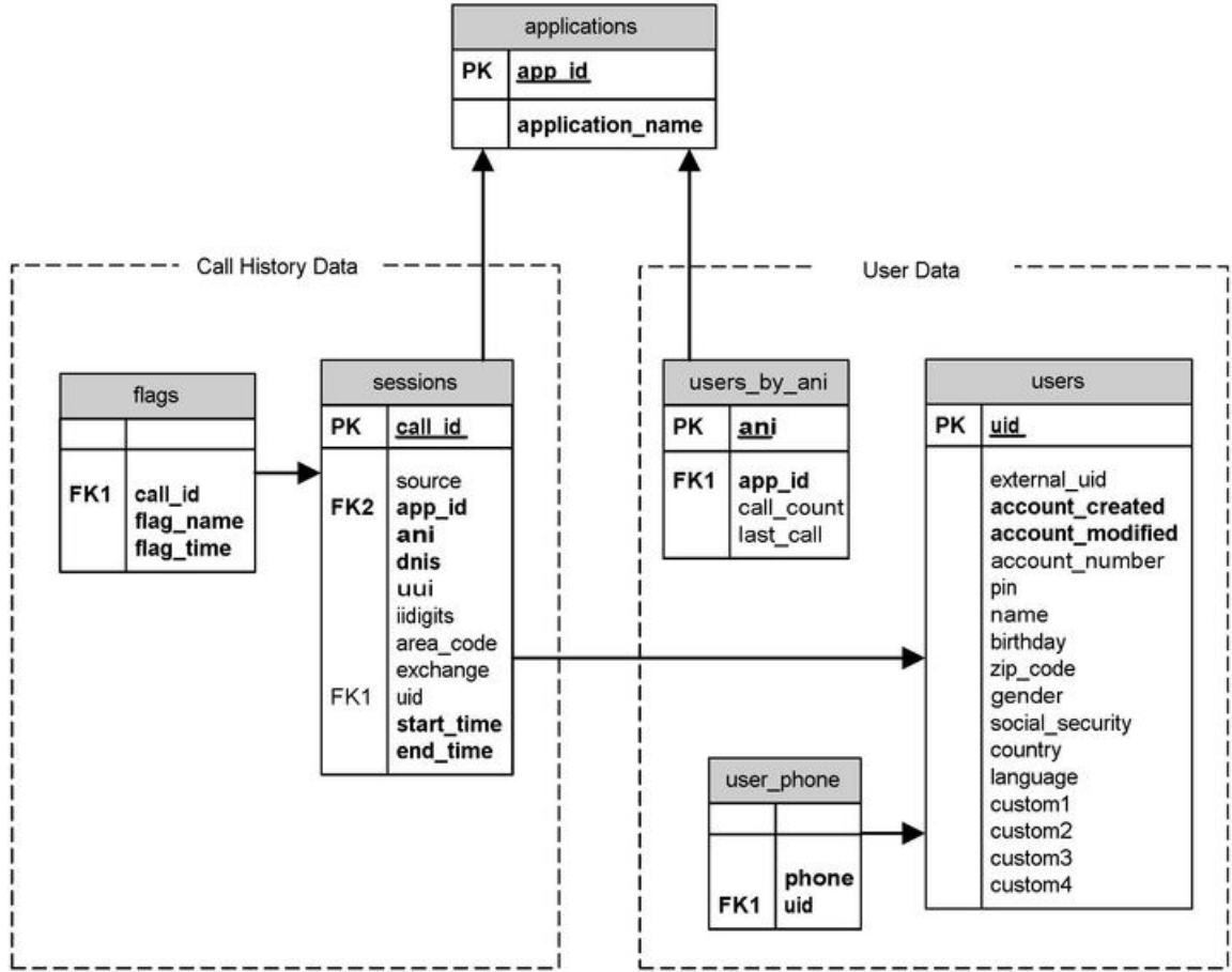
Figure 9: Database ER Diagram
