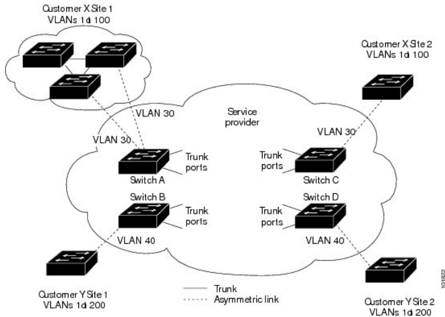
Figure 135: Layer 2 Protocol Tunneling
