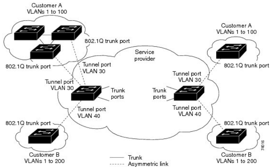
Figure 132: IEEE 802.1Q Tunnel Ports in a Service-Provider Network
