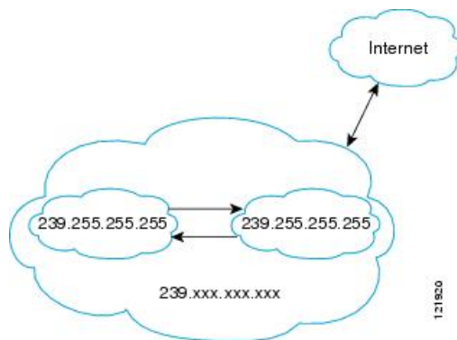
Figure 6: Address Scoping at Boundaries
