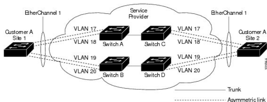
Figure 137: Layer 2 Protocol Tunneling for EtherChannels
