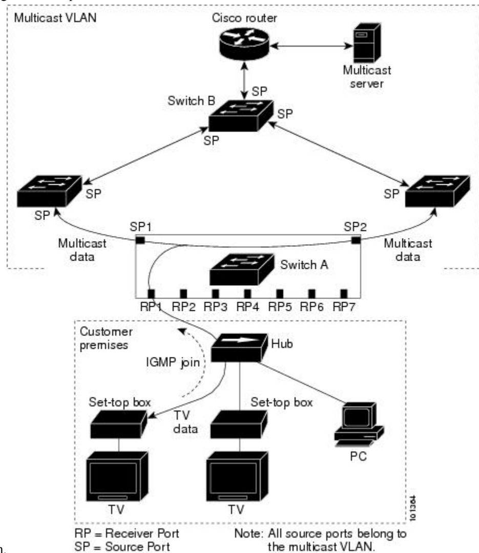
Figure 15: Multicast VLAN Registration Example
