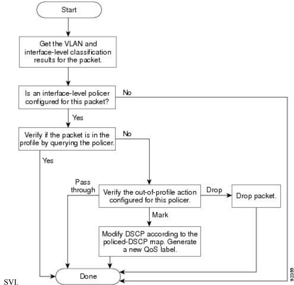
Figure 74: Policing and Marking Flowchart on SVIs
