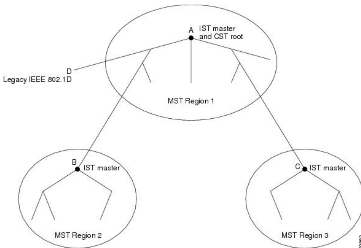
Figure 25: MST Regions, CIST Regional Root, and CST Root
