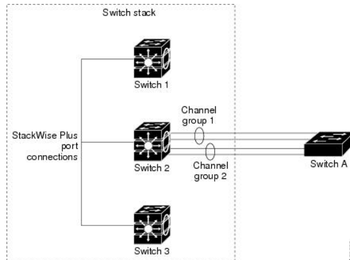
Figure 48: Cross-Stack EtherChannel
