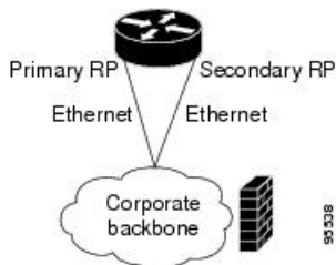
Figure 142: Dual RP Topology
