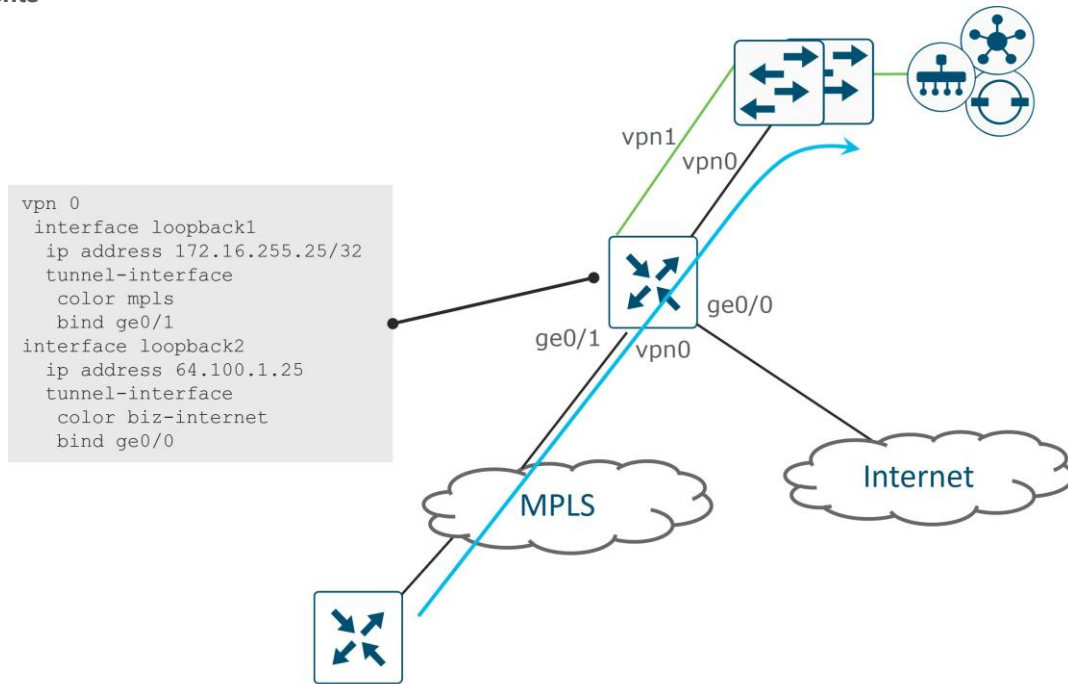
Figure 70. Loopback interface tunnel use case: SD-WAN routers need to reach on-premise control components
