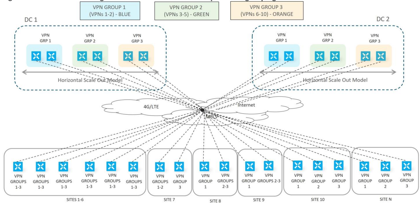
Figure 81. WAN Edge router horizontal scale example - VPN groupings
