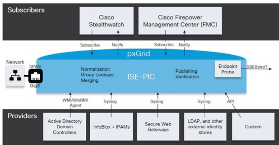
Figure 5: ISE-PIC Flow
