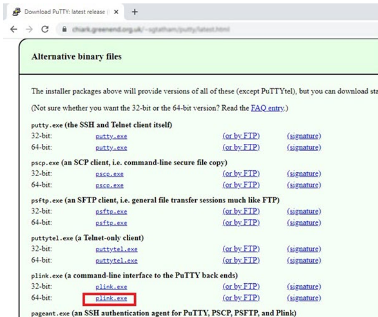
Figure 23: Download PuTTY
