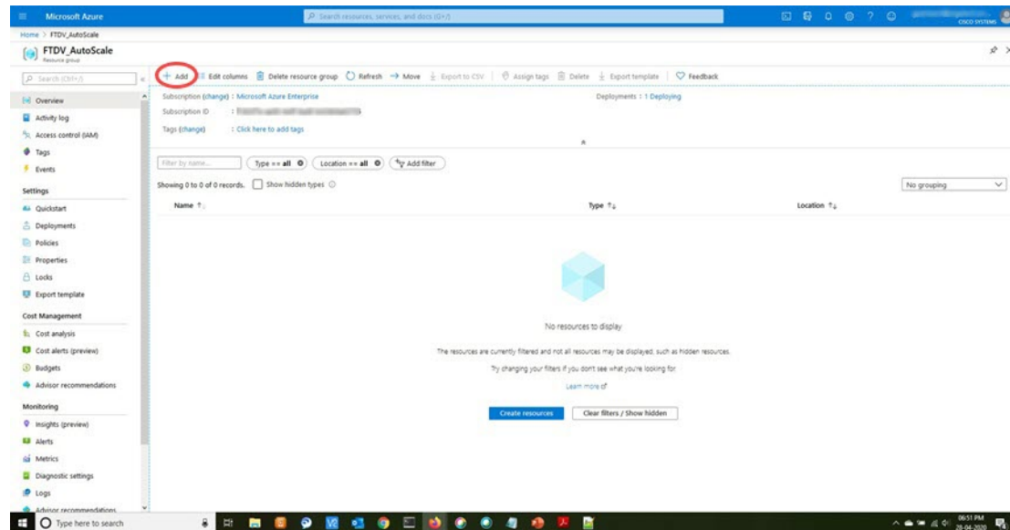
Figure 15: Azure Portal
