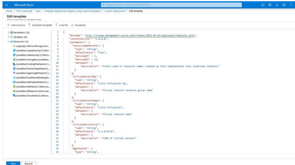
Figure 18: Edit Template
