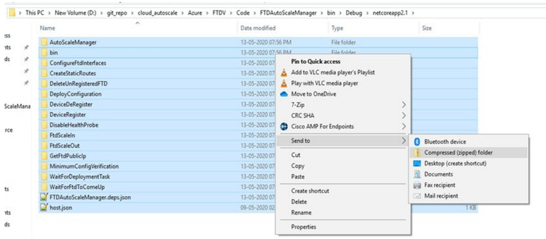
Figure 35: Build ASM_Function.zip
