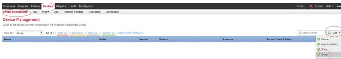
Figure 9: Device Management
