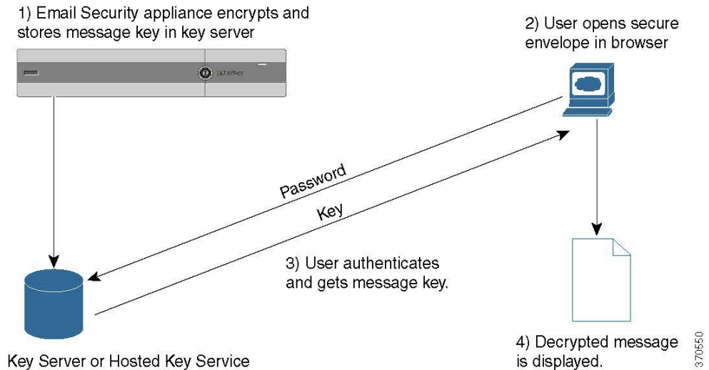
Figure 34: Encryption Workflow
