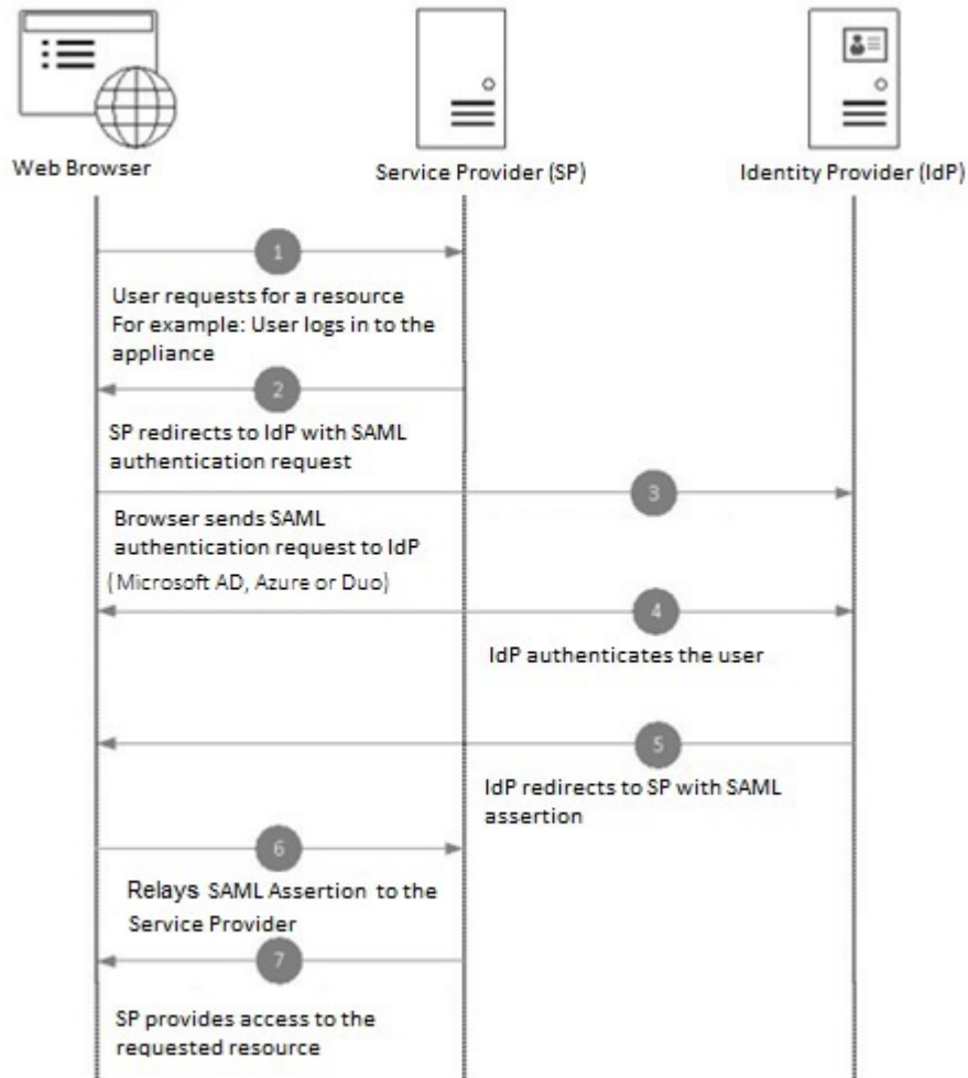
Figure 75: SAML Workflow
