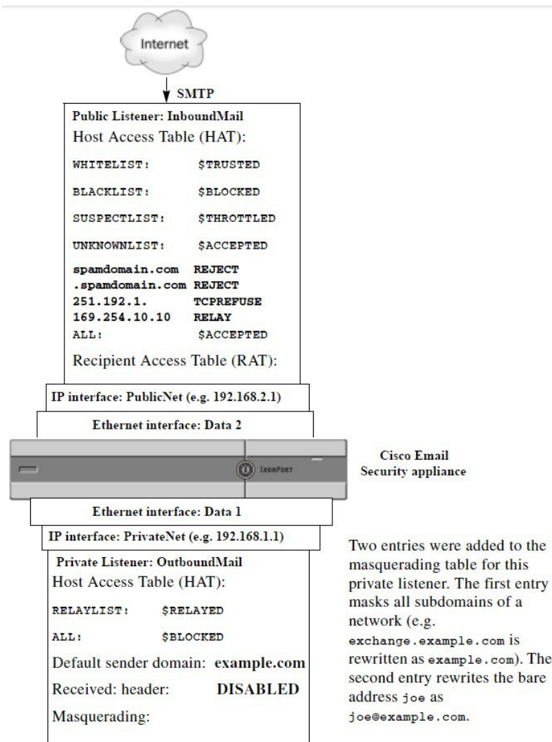
Figure 49: Masquerading Defined for a Private Listener
