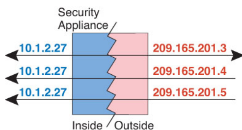
Figure 13: One-to-Many Static NAT
