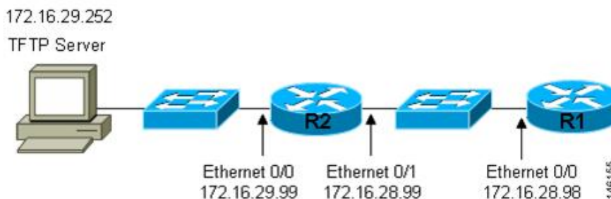
Figure 4: Example of AutoInstall That Requires a Staging Router
