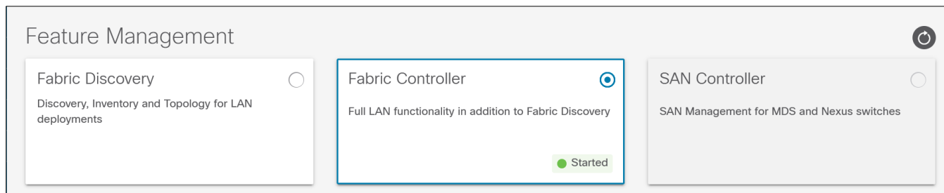
Figure 1. Feature Manager
