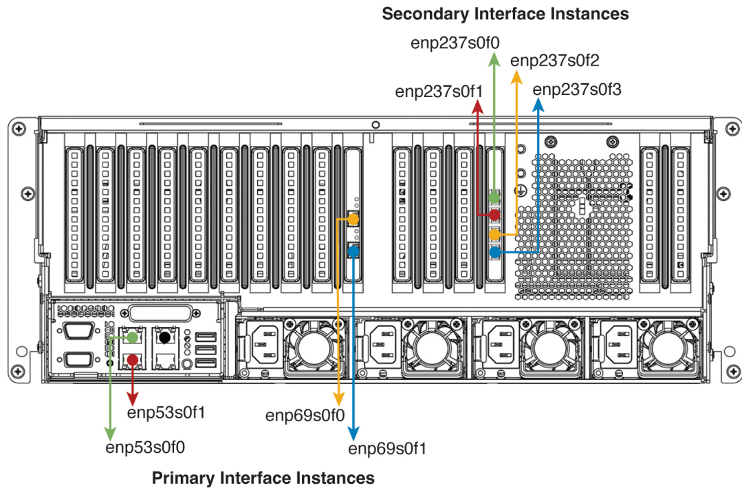
Figure 7: Recommended Cabling for 112-Core Appliance
