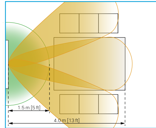
The internal microphone array with a near talker zone (green) and three beams (yellow).
