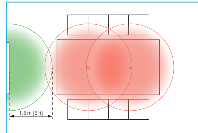
Two external microphones (red) and the internal microphone array's near talker zone (green).
