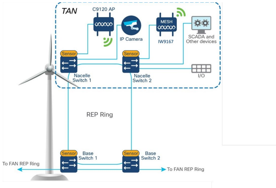
Figure 4-3 TAN HA Design, Option 2
