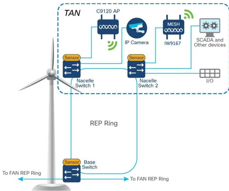
Figure 4-2 TAN HA Design, Option 1
