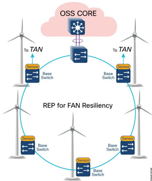
Figure 4-5 FAN Design
