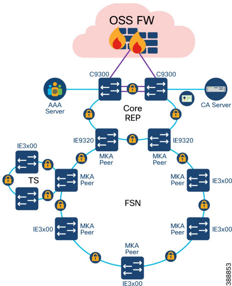
Figure 6-9 MACsec security design in turbine operator network
