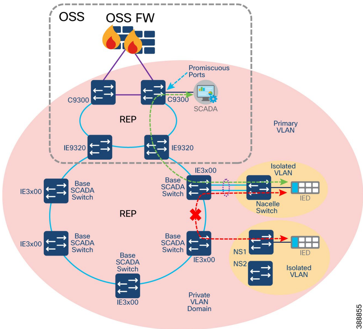
Figure 6-11 Turbine Operator SCADA Network Private VLAN Design
