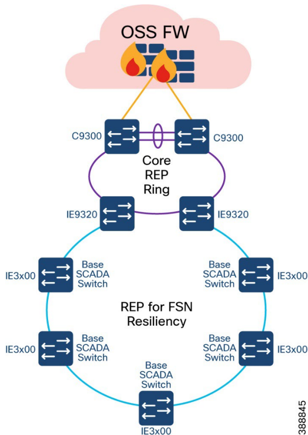
Figure 4-45 Turbine Operator Farm Area SCADA Network Design
