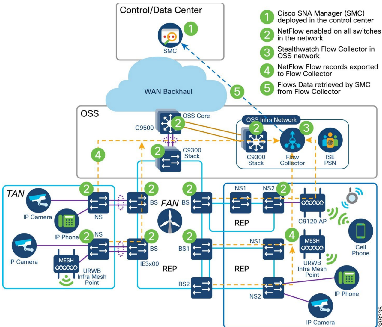
Figure 6-4 Wind Farm Secure Network Analytics (Stealthwatch) Design
