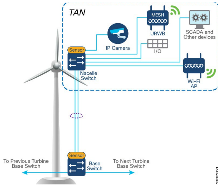
Figure 4-1 TAN Design
