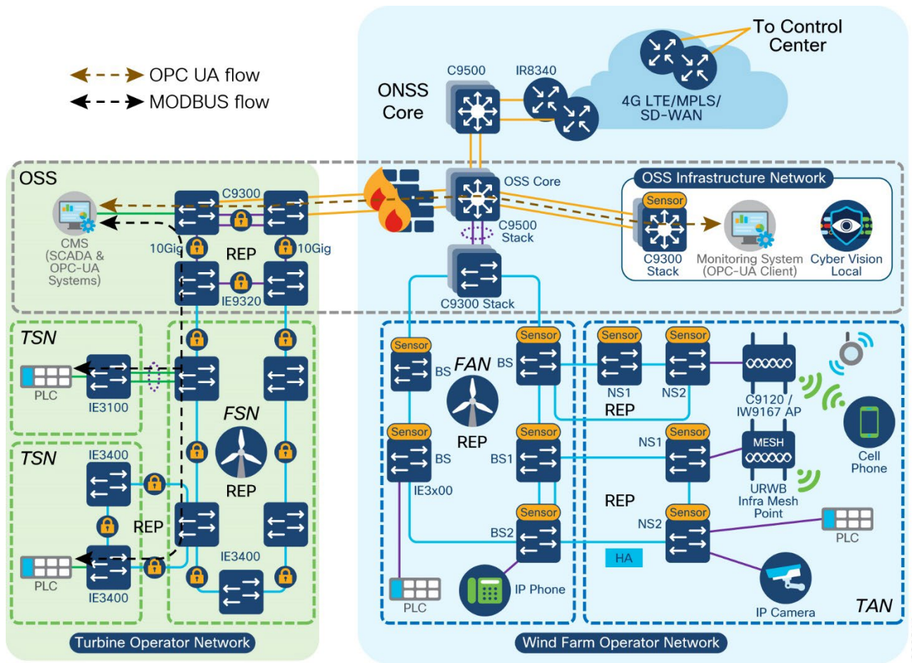
Figure 4-40 OPC UA flows between Wind Farm Asset operator and turbine operator networks
