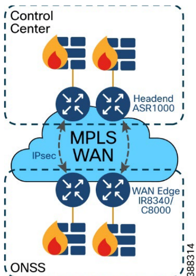
Figure 4-14 Example Wind farm WAN Backhaul
