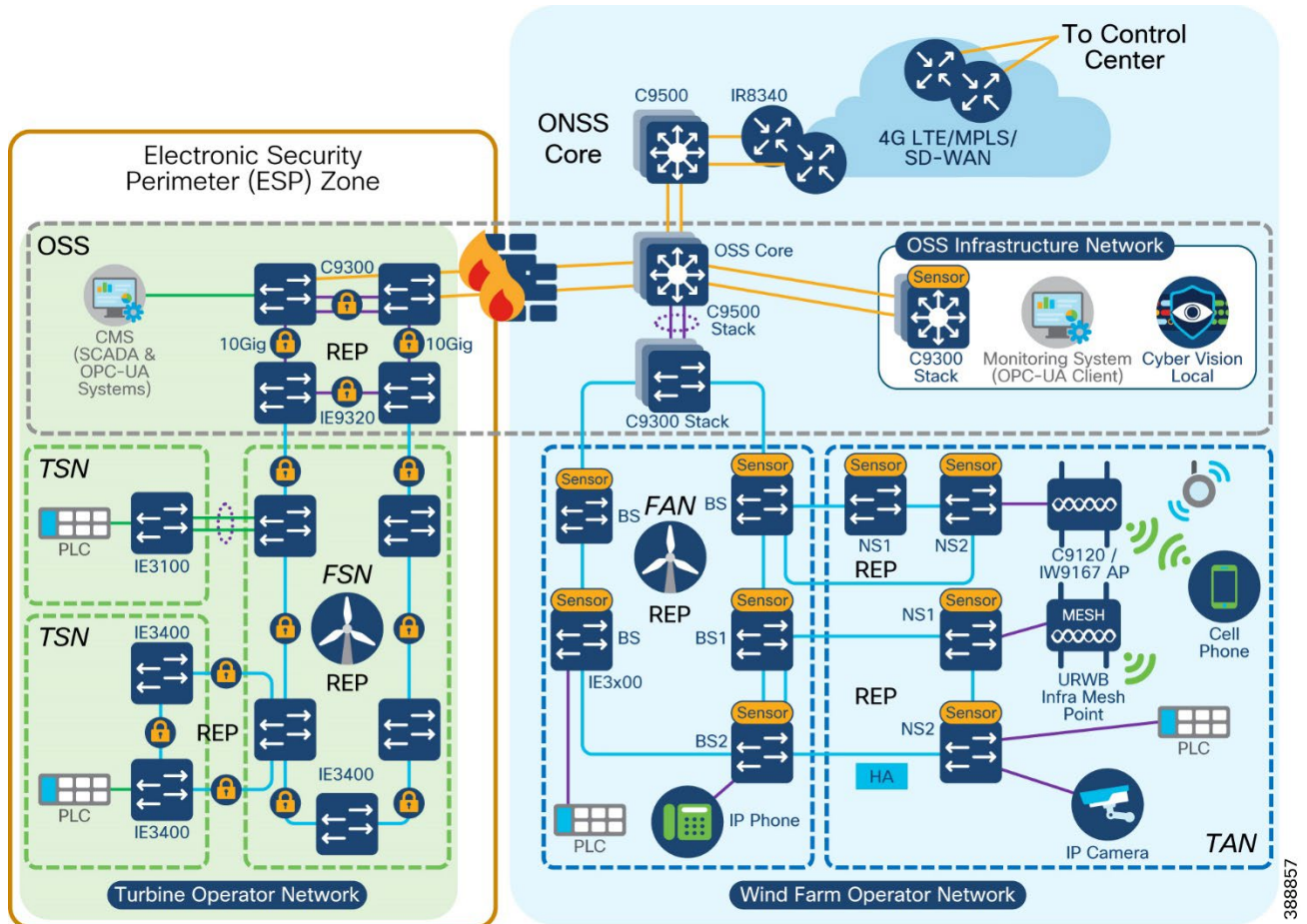
Figure 6-13 Electronic Security Perimeter in a Wind Farm with Cisco Secure Firewall
