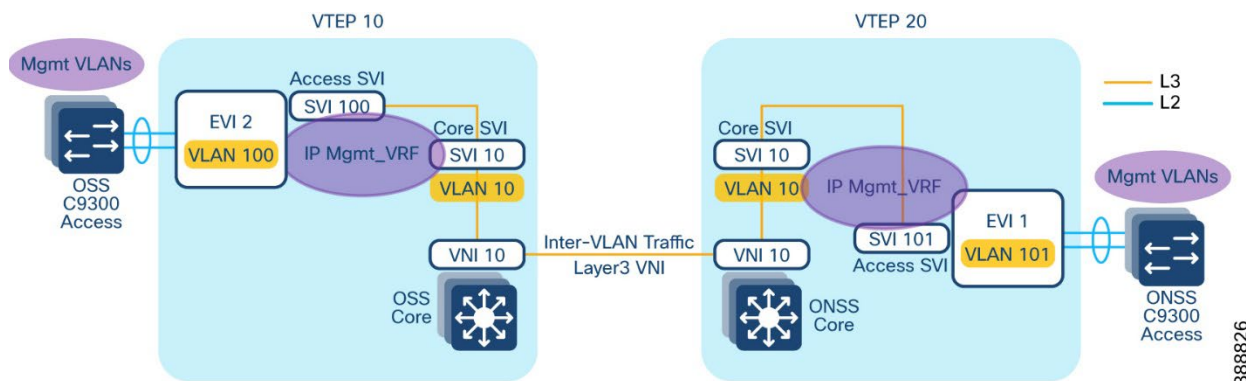
Figure 4-17 EVPN VXLAN Overlay L3VNI Routing design between OSS and ONSS Core
