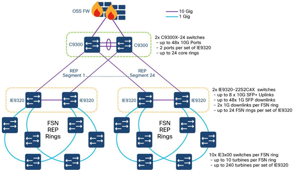
Figure 4-44 OSS Turbine Operator Aggregation Network Design
