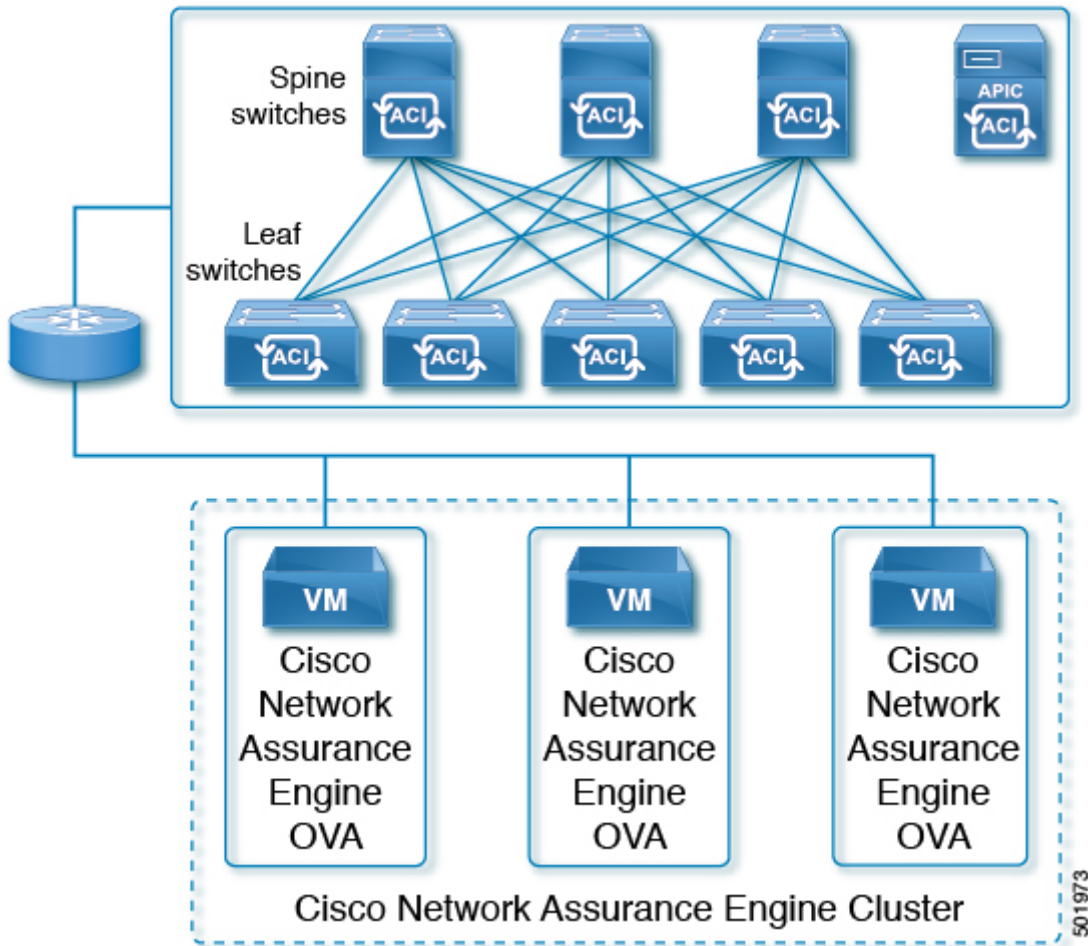
Figure 5. Out-of-Band Management Access
