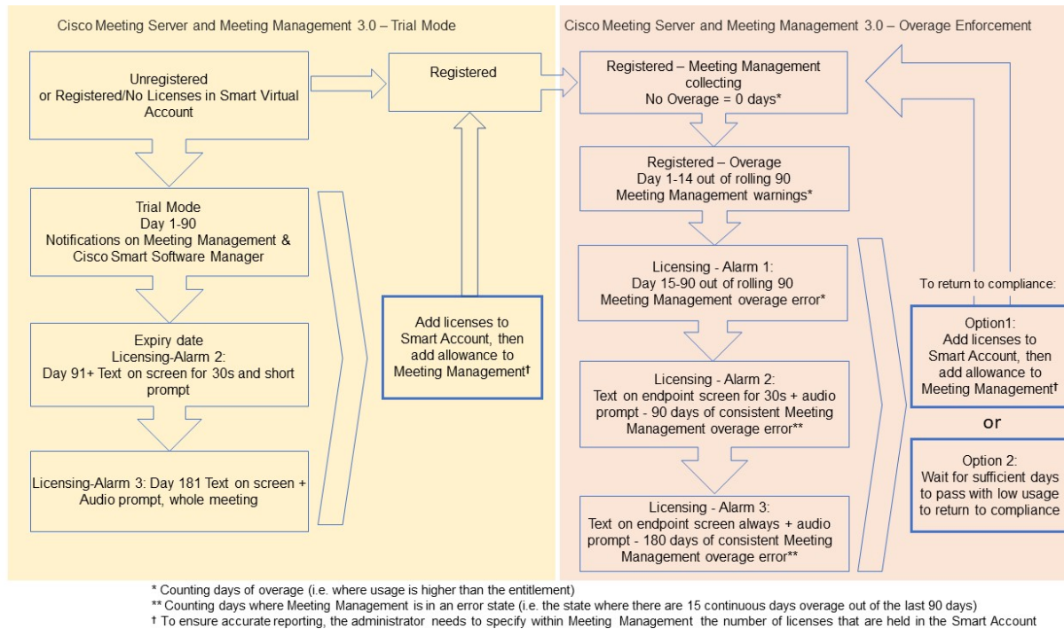
Figure 5: Cisco Meeting Server and Cisco Meeting Management Smart Licensing enforcement flow
